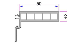
50mm Kasa Pervaz Profili P.A.099.5524.600.0.00.19
