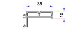
35mm Kasa Pervaz Profili P.A.099.5523.600.0.00.19
