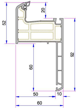
Penwood 632 Pervazlı Kasa Profili P.A.632.1200.600.2.BC.01
