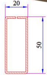
Large Coupling Profile Profili Destek Sacı 34022-12105
