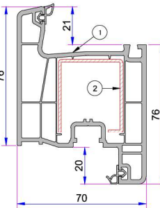
1. Dar Kanat Profili P.A.750.2111.600.0.BC.01 2. Destek Sacı (40x35x40x8) 1,2mm - 34022 - 12013 1,5mm - 34022 - 15013 2 mm - 34022 - 20013
