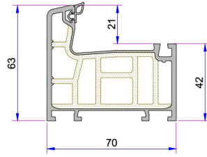
Penwood 750 Kasa Profili P.A.750.1000.600.2.BC.01
