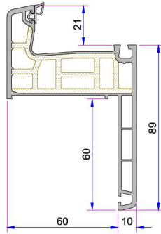
Penwood 750 Pervazlı Kasa Profili P.A.750.1200.600.2.BC.01
