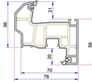
Penwood Damlalıklı Kanat Profili P.A.750.2200.600.2.BC.01
