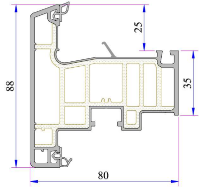
Kasa Profili P.A.883.1000.600.2.BC.01
